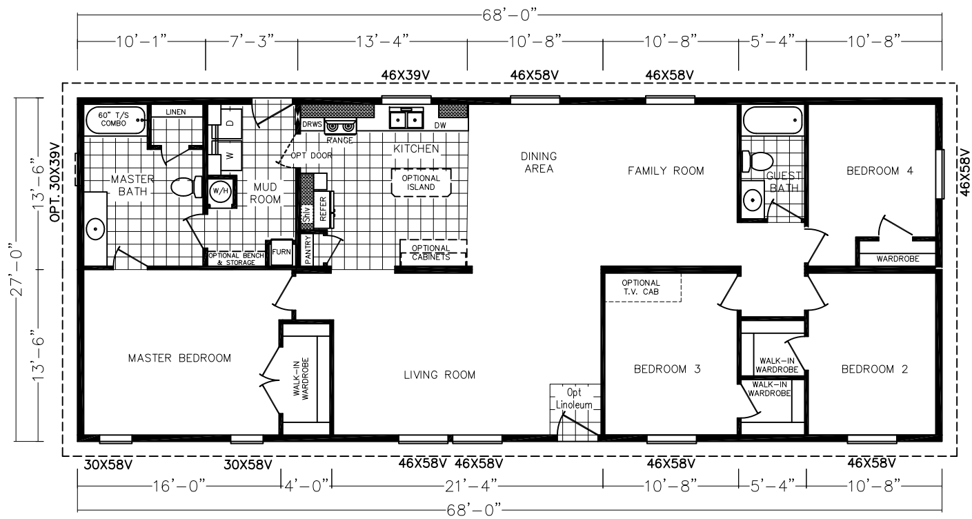
MODEL: SP-68402 F 1836 SQ. FT. 4 BEDROOM 2 BATH
