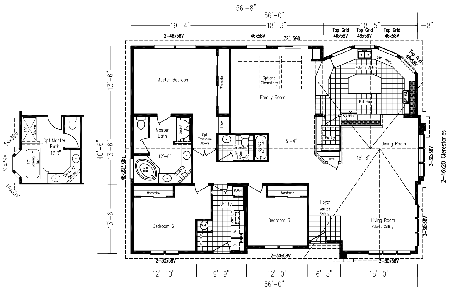
Model: KMCK-56881 K 2229 Sq. Ft. 3 Bedroom 2 Bath
