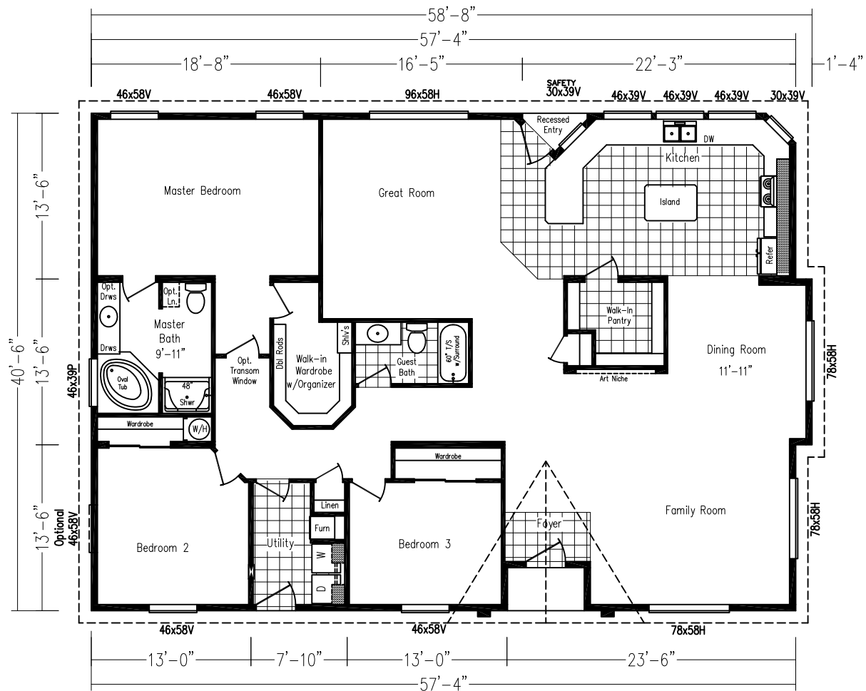
Model: KMCK-5701 K (2305 Sq. Ft. + 31 Sq. Ft. Porch) 3 Bedroom 2 Bath
