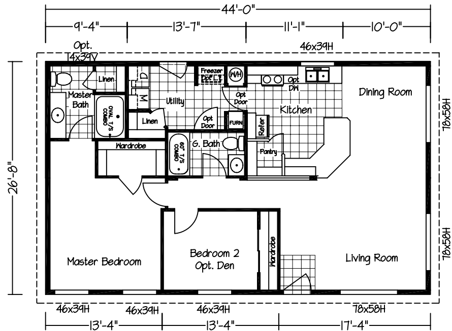
Model: KLTD-44092 1173 Sq. Ft. 2 Bedroom 2 Bath
