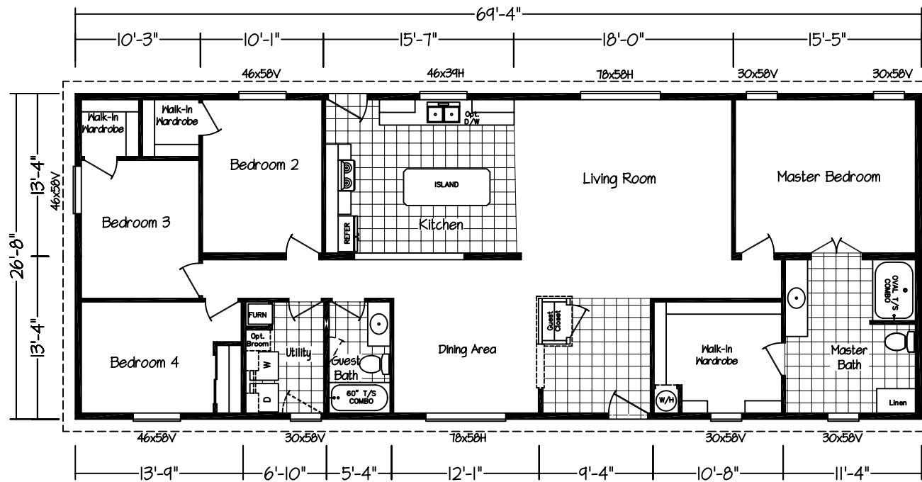
Model: KLTD-69207 1848 Sq. Ft. 4 Bedroom, 2 Bath
