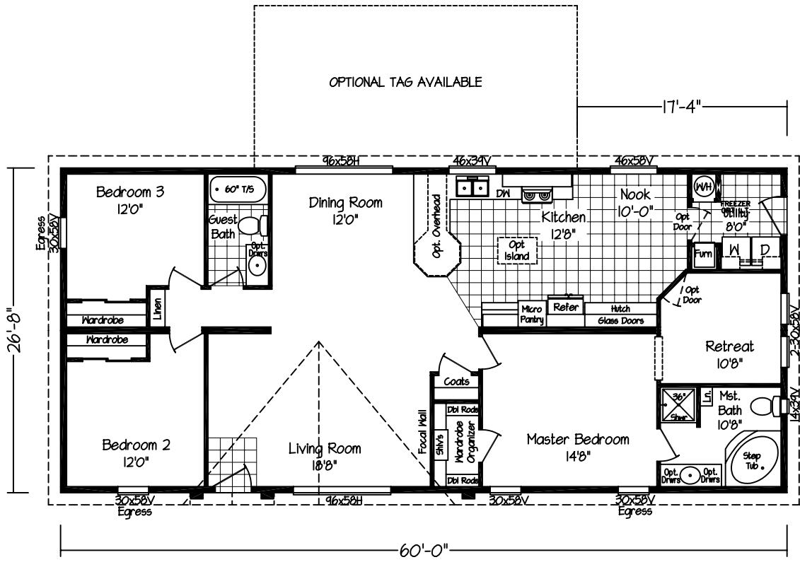
Model: KMCK-60862 1600 Sq. Ft. 3 Bedroom 2 Bath W/Retreat
