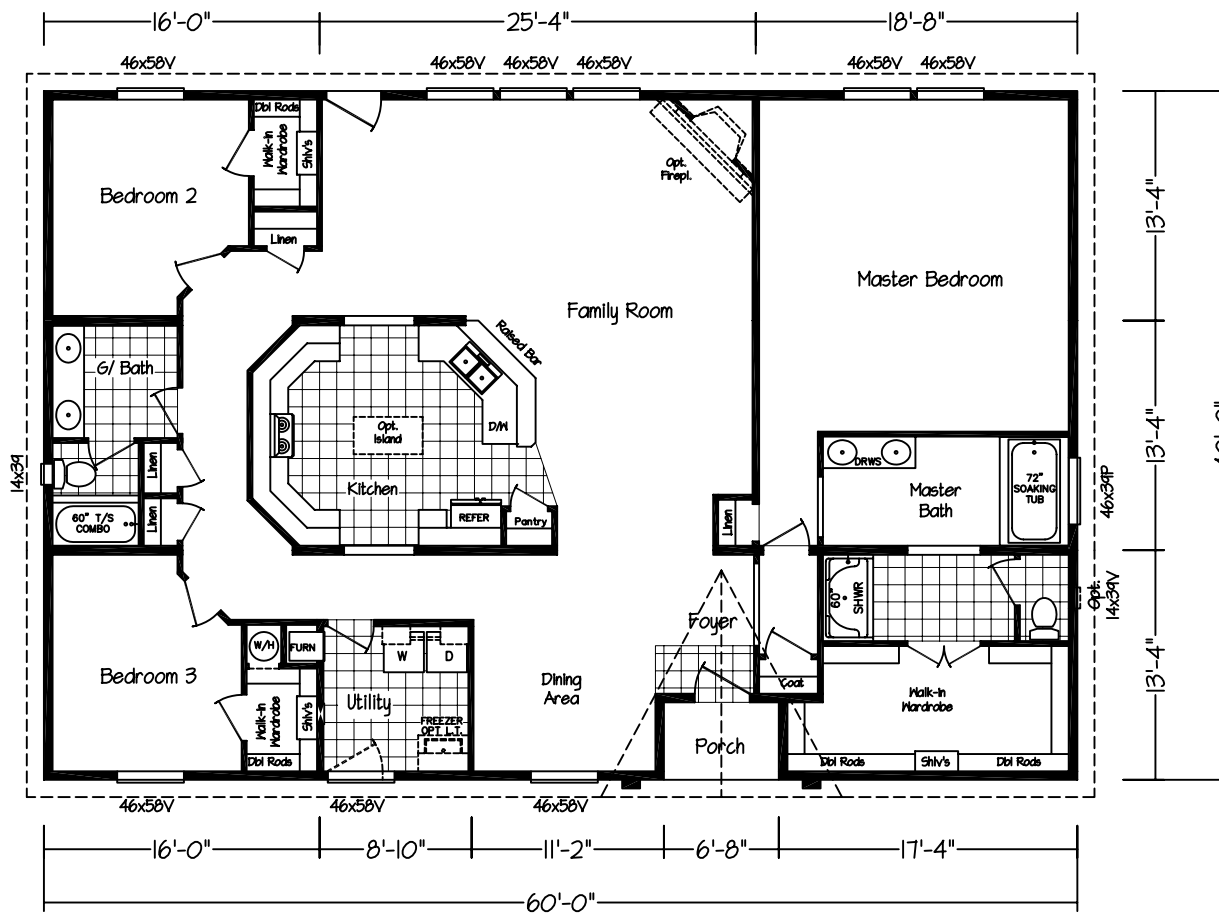
Model: KMCK-60883 2370 Sq. Ft. (Does not include porch) 3 Bedroom 2 Bath
